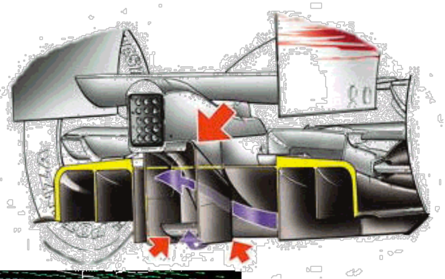
Toyota TF109 - rear diffuser design
